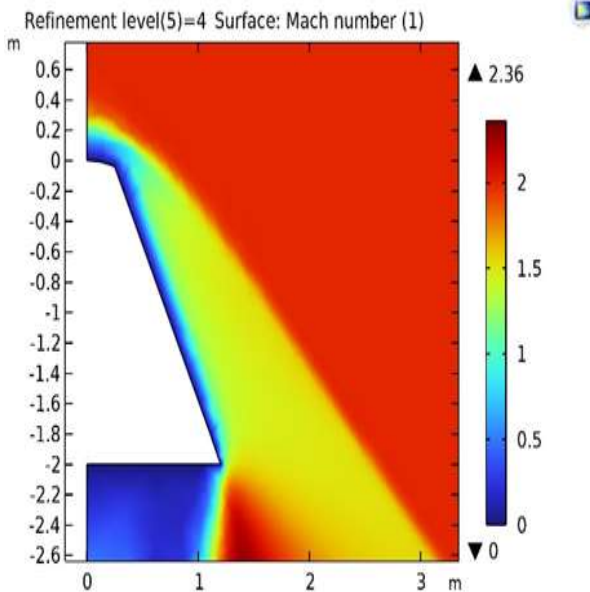
Fig. 8. Mach number distribution around the body, highlighting compressibility effects and shock formation.
