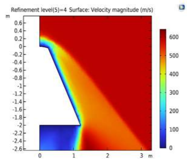
Fig.3. Velocity magnitude contour around the shape, illustrating the deceleration at the stagnation point and acceleration of the flow along the body surface.
