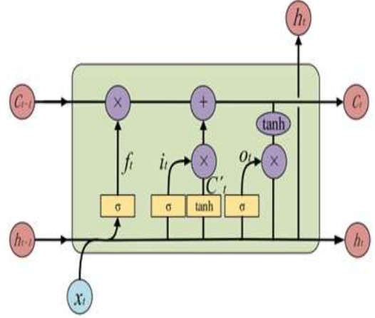
Fig. 5. The structure of the classic LSTM.
