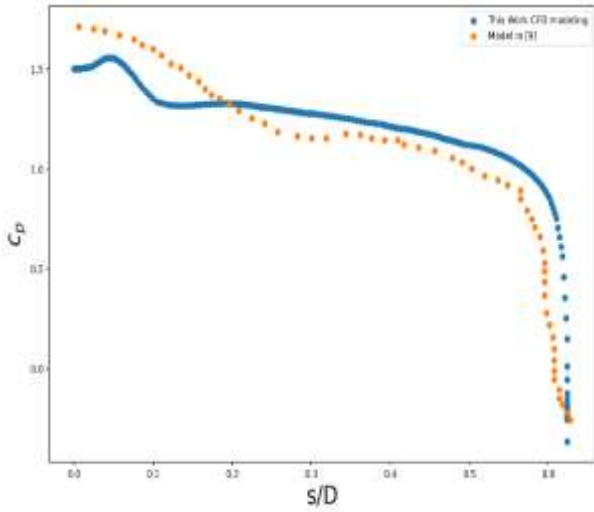
Fig. 4. Comparison of surface pressure coefficient ( C_p ) distribution along the normalized surface coordinate ( s/D ) between the present CFD modeling and the reference data from Mehta [19].
