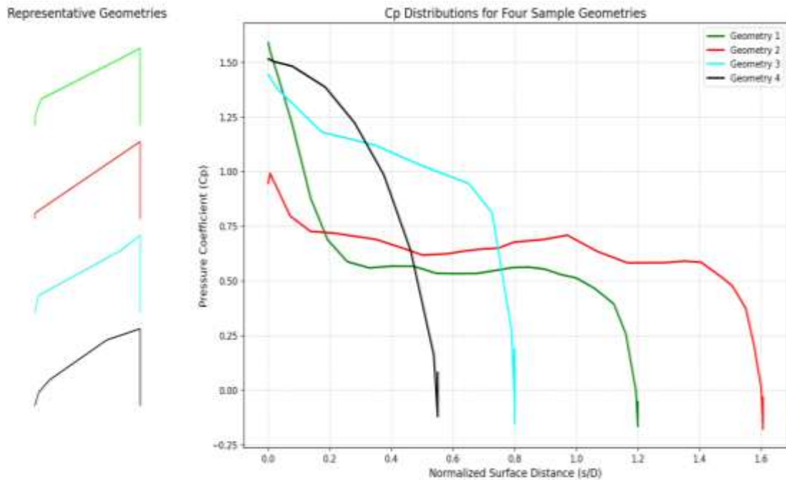
Fig. 6. four representative configurations (left) together with their corresponding surface pressure coefficient ( C_p ) distributions as a function of normalized surface distance.
