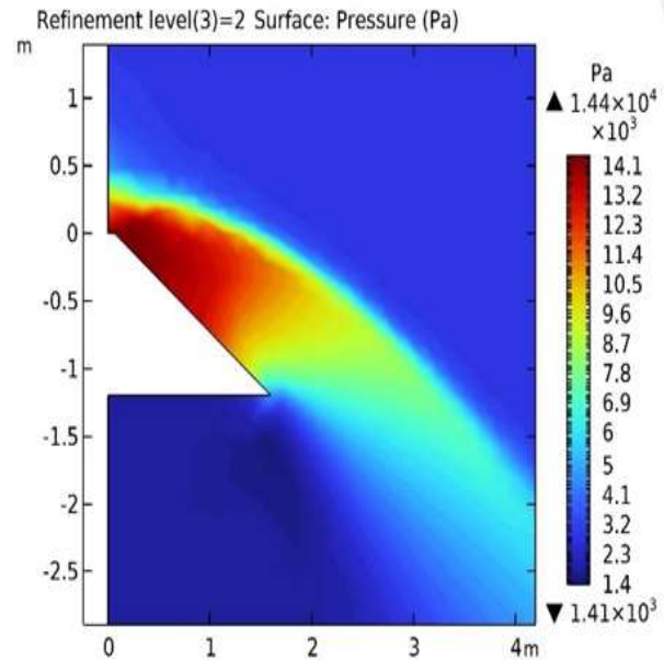
Fig. 9. a) the predicted pressure coefficient ( C_p ) values with those obtained from CFD simulations for the represented geometry b) Surface pressure distribution (Pa) from CFD simulation for a random geometry ( R=1.3m , L=1.2 , \alpha=52^\circ , \beta=52^\circ , D=1.6m , x=0.2m ).
