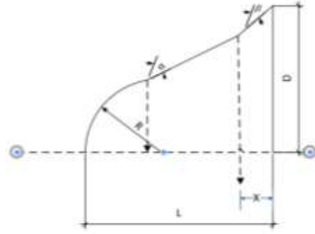
Fig. 1. Parametric definition of the sphere-cone geometry.
