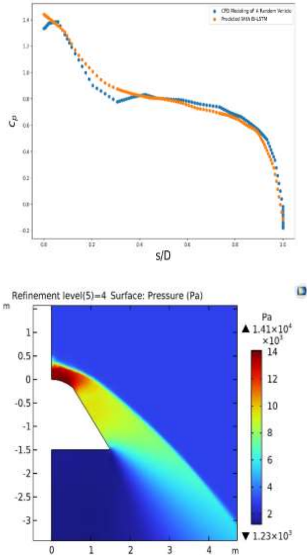
Fig. 11. a) the predicted pressure coefficient ( C_p ) values with those obtained from CFD simulations for the represented geometry b) Surface pressure distribution (Pa) from CFD simulation for a random geometry ( R=0.93m , L=1.5 , \alpha=36^\circ , \beta=35^\circ , D=1.5m , x=0.2m ).
