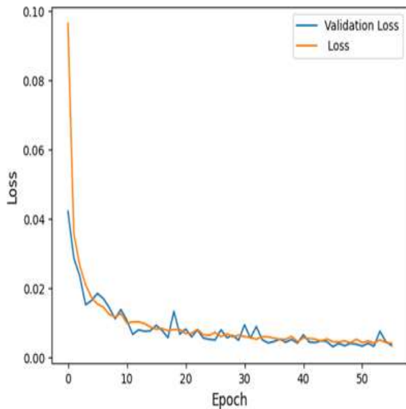
Fig. 10. Training and validation loss curves of the BiLSTM model over 55 epochs.
