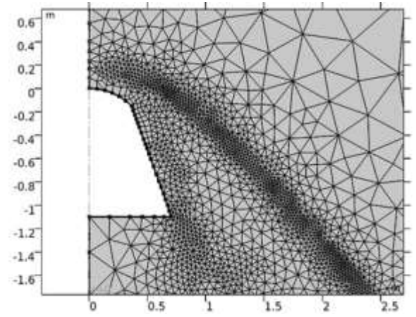
Fig.2. Adaptive triangular mesh used for the 2D axisymmetric CFD simulation. The mesh is refined near the stagnation point and flare region to ensure accurate resolution of flow gradients in high Mach number conditions.
