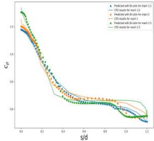
Fig. 12. Comparison of BiLSTM-predicted and CFD-computed pressure coefficient distributions for a representative geometry at Mach 1.5, Mach 2.0, and Mach 2.5 for a random geometry ( R=1.3\text{m} , L=1.2 , \alpha=18^\circ , \beta=18^\circ , D=1\text{m} , x=0.2\text{m} ).
