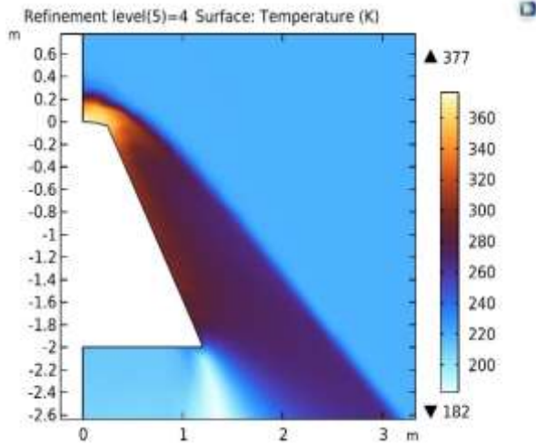
Fig.7. Temperature contour around the body, showing thermal gradients resulting from shock compression and viscous effects. The highest temperatures appear near the stagnation region due to strong flow deceleration and compress.
