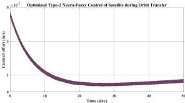
Fig. 5. Control signal generated by the optimized Type-2 neuro-fuzzy controller under Hall-effect thruster fault conditions.
