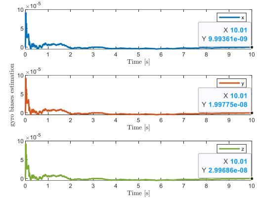
Fig. 4. Estimated gyroscope biases in scenario 1.
