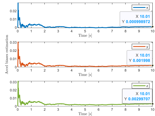
Fig. 5. Estimated accelerometer biases in scenario 2.
