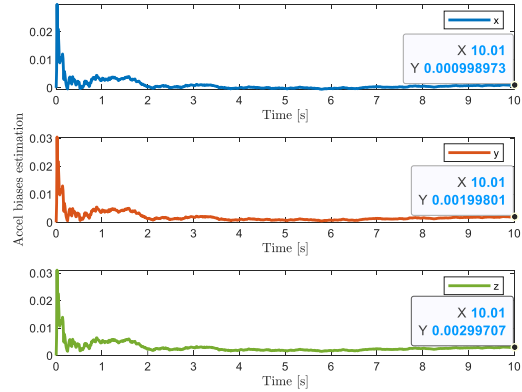
Fig. 3. Estimated accelerometer biases in scenario 1.
