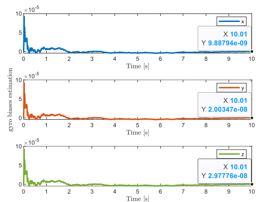
Fig. 6. Estimated gyroscope biases in scenario 2.
