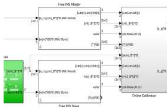
Fig. 2. Outputs of the reference and dependent systems and inputs to the bias estimation algorithm.
