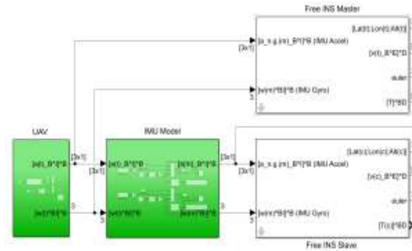
Fig. 1. Modeling of reference and dependent system inputs
