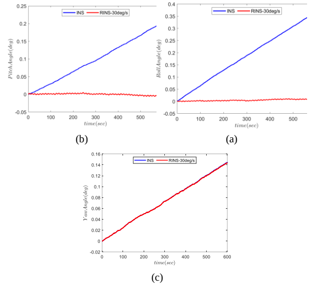
Fig. 1. Bias error of the attitude during sensor rotation about the z-axis (a) Roll angle, (b) Pitch angle, (c) Yaw angle.
