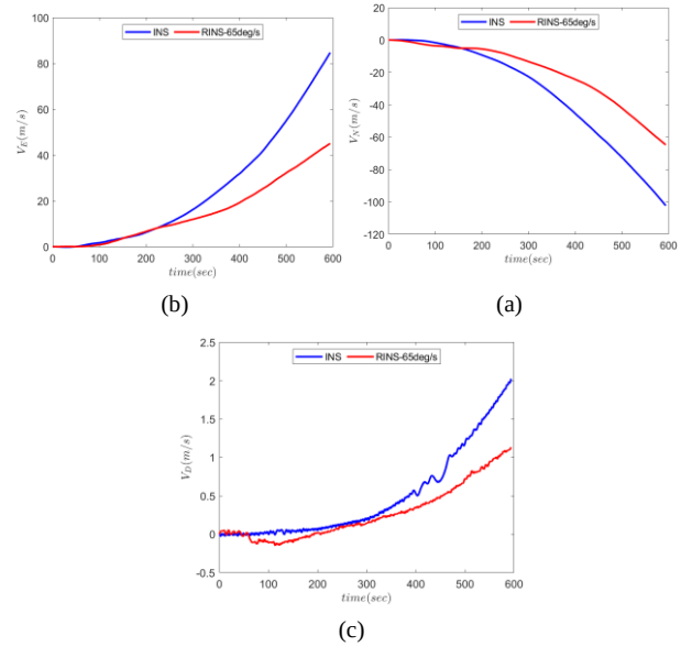
Fig. 7. Experimental Test error of the Velocity during sensor rotation about the z-axis: (a) Velocity along North, (b) Velocity along East, (c) Velocity along Down.
