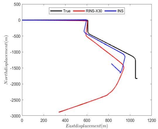
Fig. 10. North and East displacement errors during sensor rotation about the x-axis.
