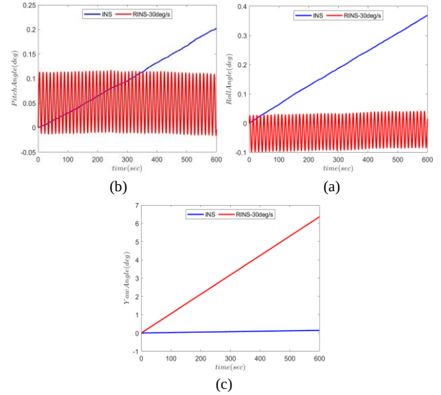
Fig. 7. Combined error of the attitude during sensor rotation about the z-axis: (a) Roll angle, (b) Pitch angle, (c) Yaw angle.
