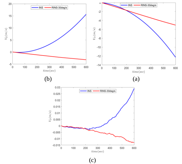
Fig. 8. Combined error of the Velocity during sensor rotation about the z-axis: (a) Velocity along North, (b) Velocity along East, (c) Velocity along Down.
