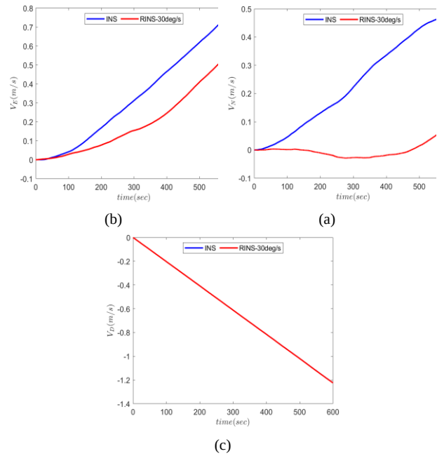
Fig. 4. Scale factor error of the Velocity during sensor rotation about the z-axis: (a) Velocity along North, (b) Velocity along East, (c) Velocity along Down.
