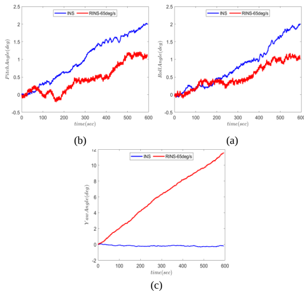
Fig. 6. Experimental Test error of the attitude during sensor rotation about the z-axis: (a) Roll angle, (b) Pitch angle, (c) Yaw angle.
