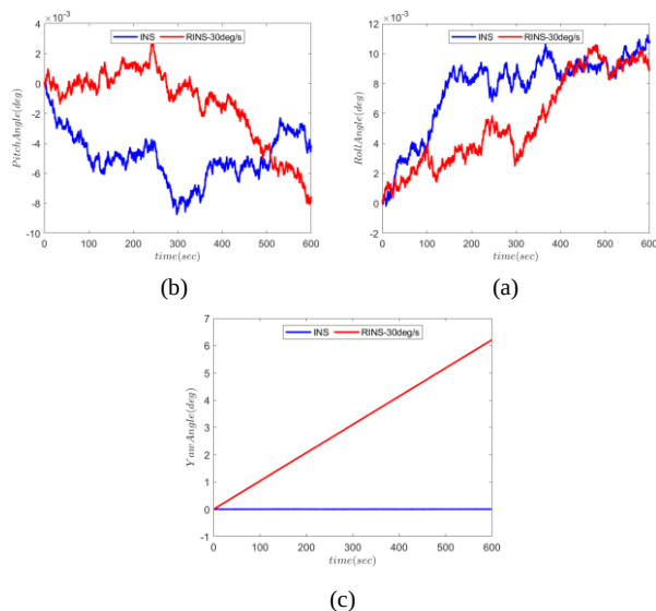
Fig. 3. Scale factor error of the attitude during sensor rotation about the z-axis: (a) Roll angle, (b) Pitch angle, (c) Yaw angle.
