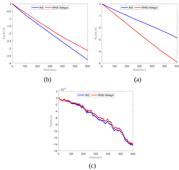
Fig. 6. Installation error of the Velocity during sensor rotation about the z-axis: (a) Velocity along North, (b) Velocity along East, (c) Velocity along Down.
