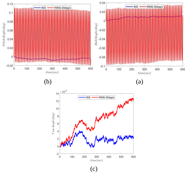
Fig. 5. Installation error of the attitude during sensor rotation about the z-axis: (a) Roll angle, (b) Pitch angle, (c) Yaw angle.
