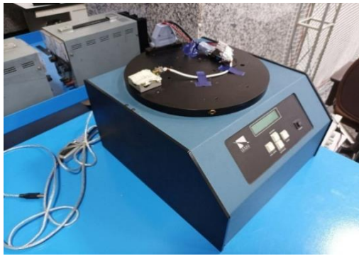
Fig. 5. Experimental Setup.
