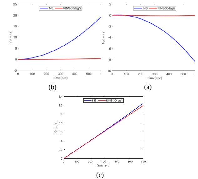
Fig. 2. Bias error of the Velocity during sensor rotation about the z-axis: (a) Velocity along North, (b) Velocity along East, (c) Velocity along Down.
