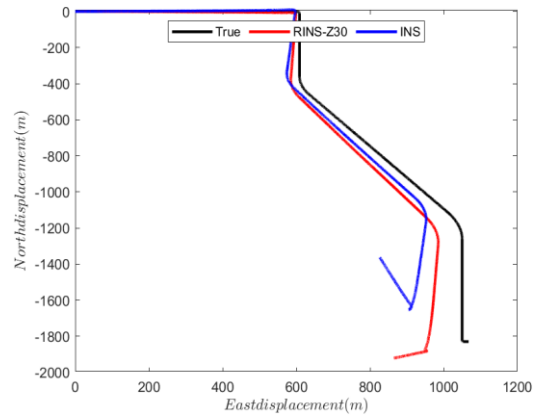
Fig. 9. North and East displacement errors during sensor rotation about the z-axis.
